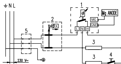
Electric installation
